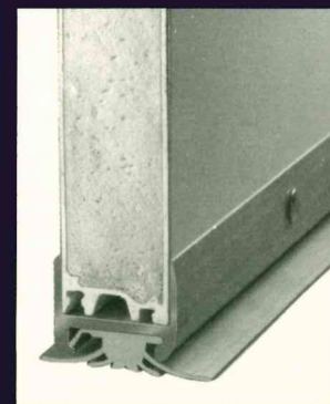
Rigid bottom U-channel with replaceable vinyl bottom seal
