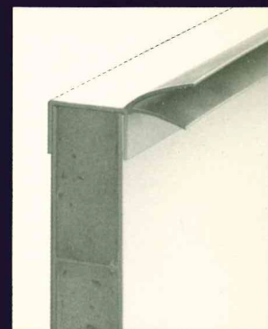
Dual durameter PVC top seal. Rigid section of seal forms cap at top of door to strengthen top panel
